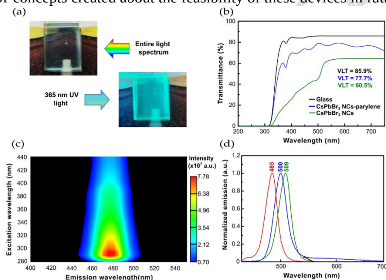
Figure 1 - Encapsulation of CsPbBr 3 NCs thin films with parylene type C: (a) coated glass sample under the entire light spectrum and 365 nm UV light; (b) impact on the light being transmitted through the glass (black line), when coated with CsPbBr 3 NCs thin film (green line), and with the composite film of NCs-polymer (blue line); (c) contour plot of the photoluminescence emission intensity at different excitation wavelengths; (d) normalized emission spectra of CsPbBr 3 NCs in solution (blue line), CsPbBr 3 NCs thin film (green line), and CsPbBr 3 NCs -parylene thin film (red line). [5]
