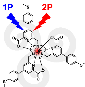
Figure 3. The structure of target Ln(III) complexes of a new tacn-based ligand with thioanisoly-picolinate antennae.
