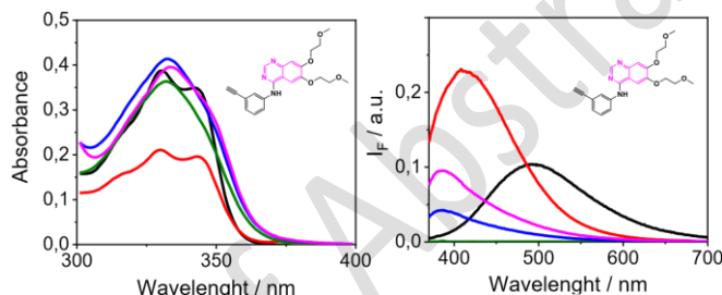
Figure 1. Absorption and fluorescence spectra ( \lambda_{exc} = 340 nm) of ERL in solution [MeCN (black), CyH (red) and PBS (green)] and in the presence of HSA (blue) and HAG (magenta).
