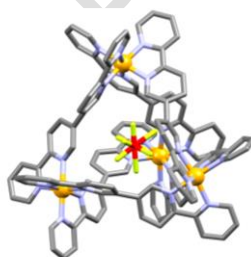
Figure 1. X-ray molecular structure of the tetrahedral [\text{Cr}^{\text{III}}_4\text{L}_6]^{12+} molecular cage ( \text{L} = 2,2':5',5'':2'',2''' -quaterpyridine) encapsulating a \text{PF}_6 anion.
