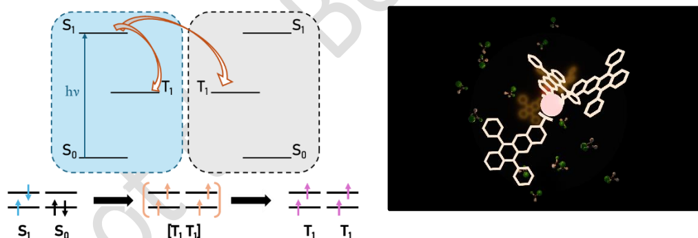
Figure. a) simplified Jablonsky-Perrin diagram and schematic representation of singlet-fission process; b) schematic representation of target lanthanide complex.
