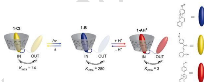
Figure 1 Control over the self-inclusion complex affinity through the trans-chalcone 1-Ct (Moderate Affinity)-Hemiketal 1-B (high Affinity) or Flavylium 1-AH + (low affinity) interconversion using only light or light and pH stimuli, respectively.
